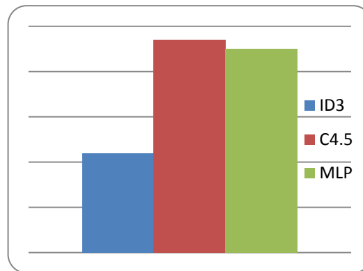
Figure 6: Prediction Accuracy
