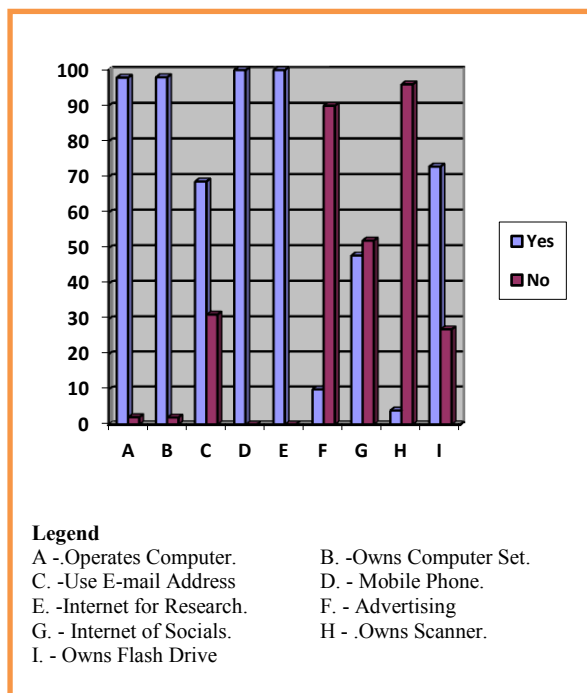
Figure 1: ICT Usage
