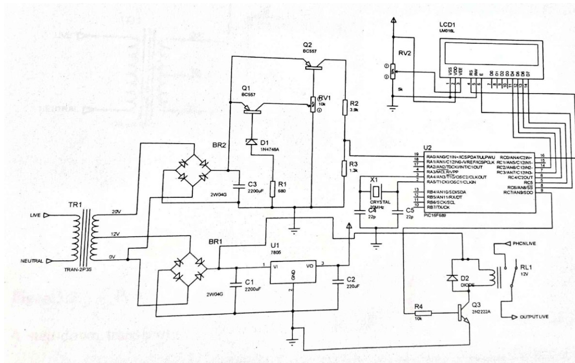
Figure 2: Circuit Diagram
