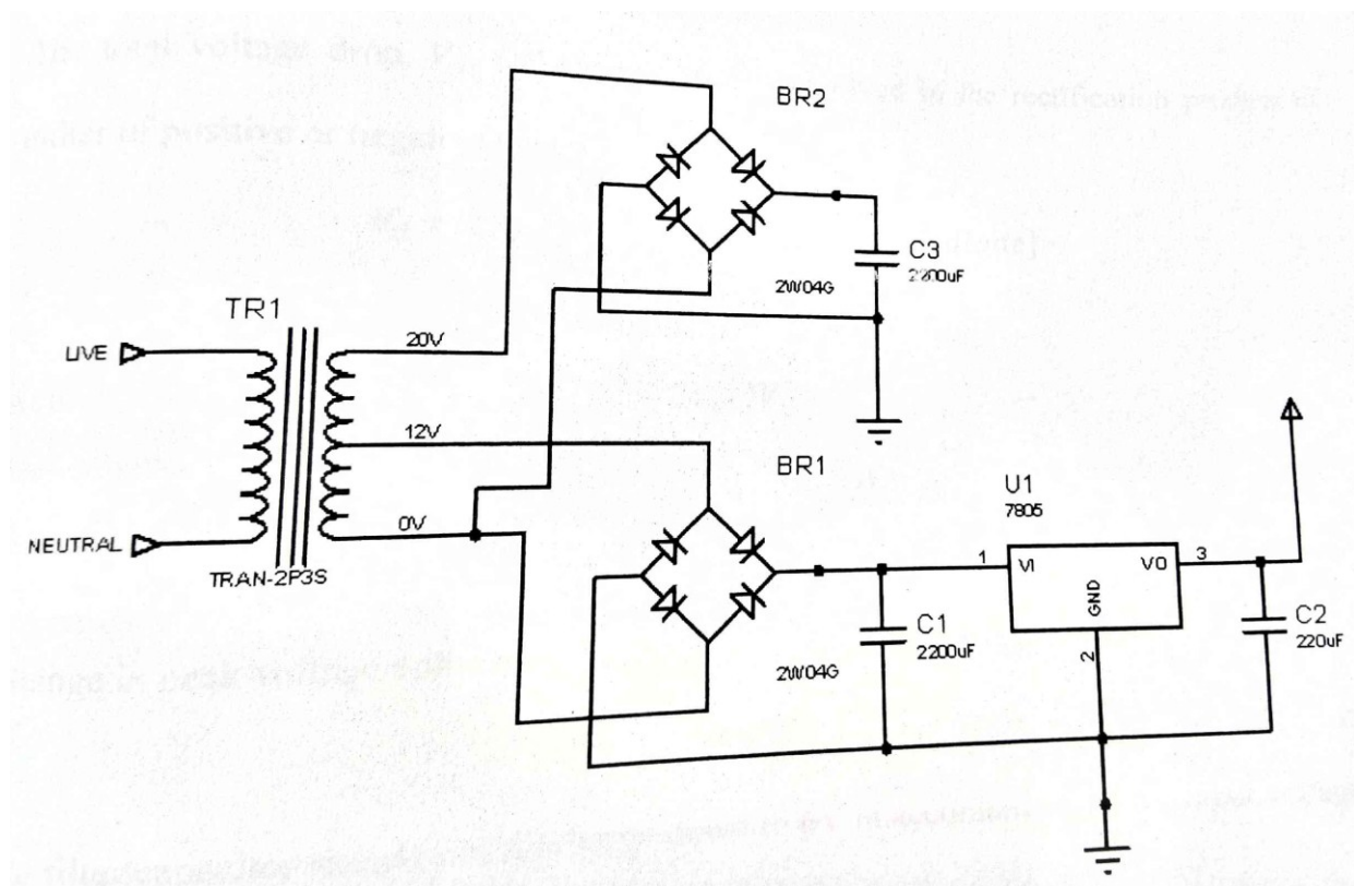
Figure 1: Power Supply Circuit
