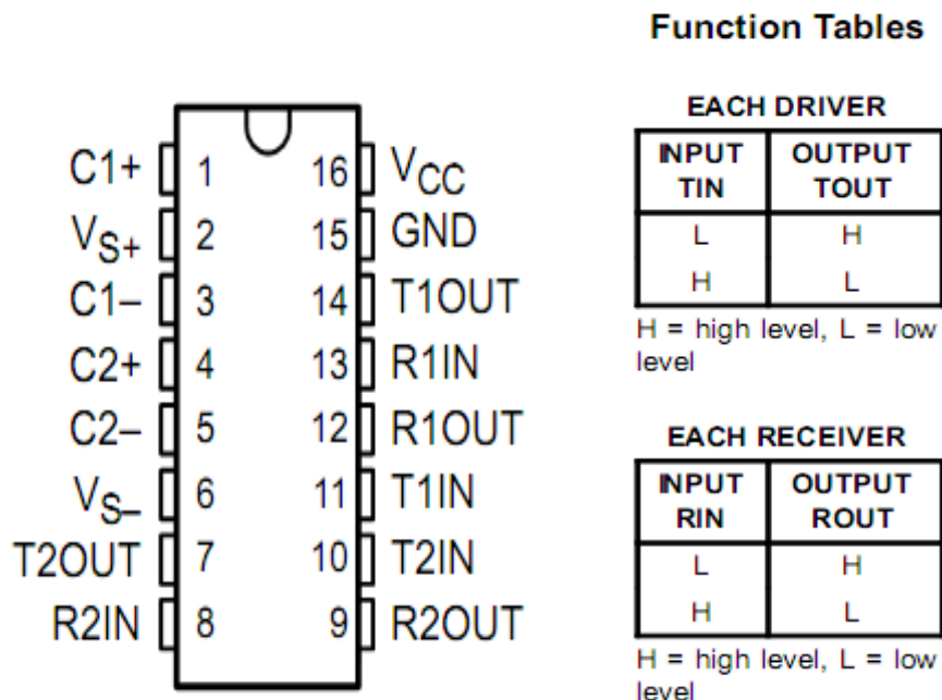
Fig 4: Pin Diagram of MAX232
