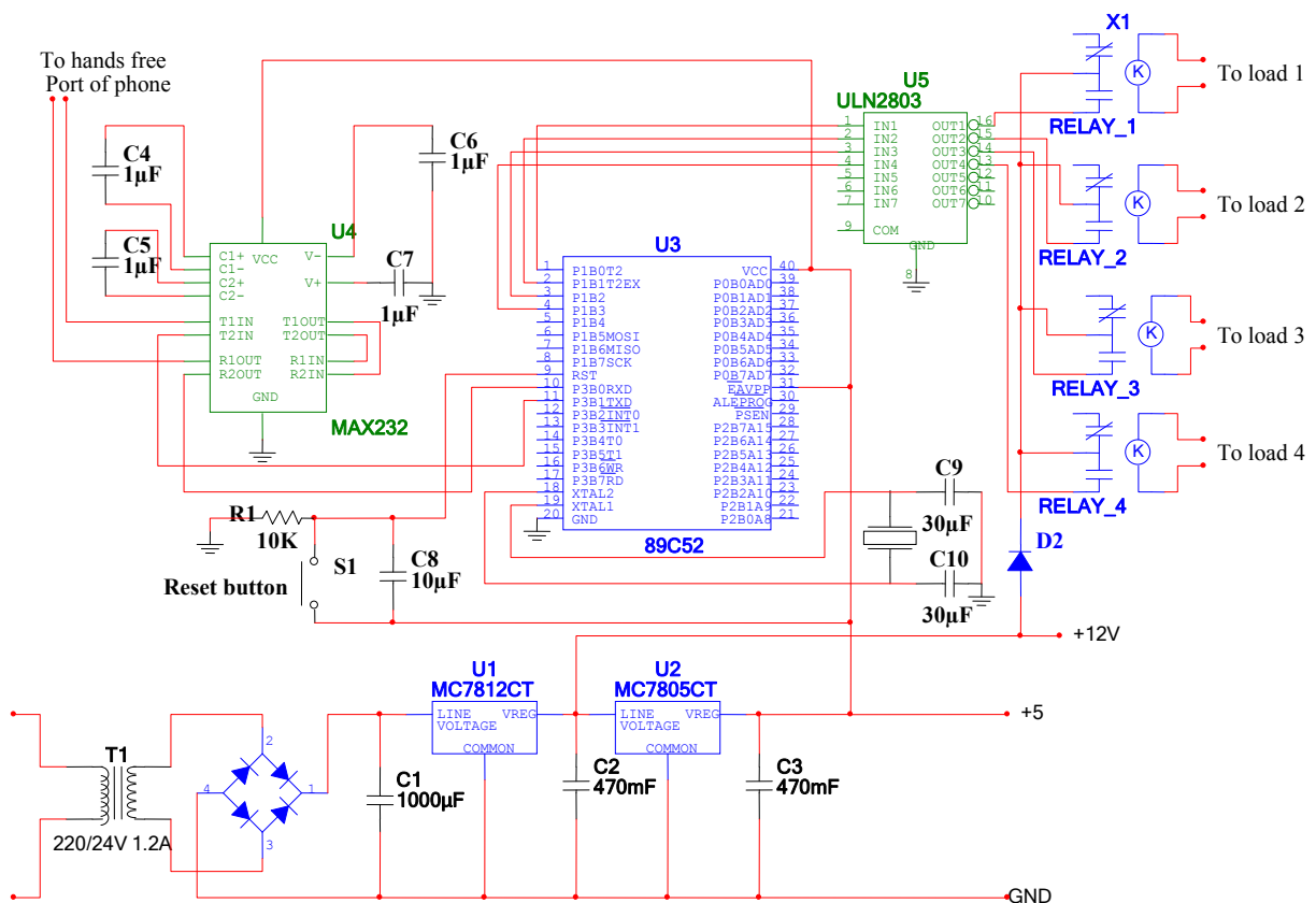
Fig 8: Complete Circuit Diagram of a SMS Operated Switch/SMS Appliance Control
