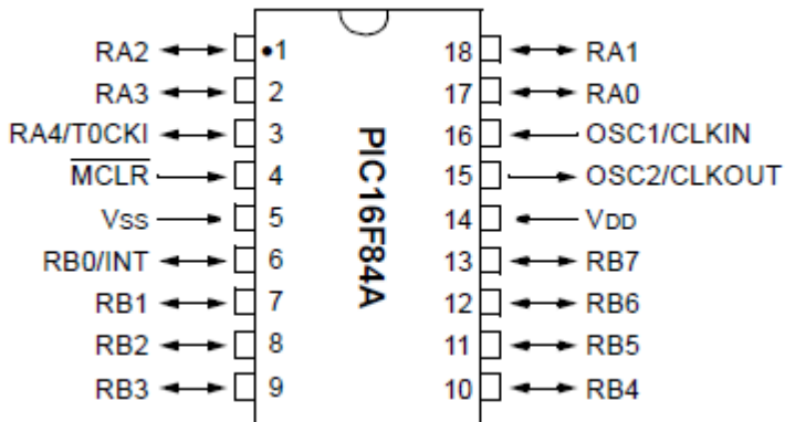
Fig 3: Microcontroller
